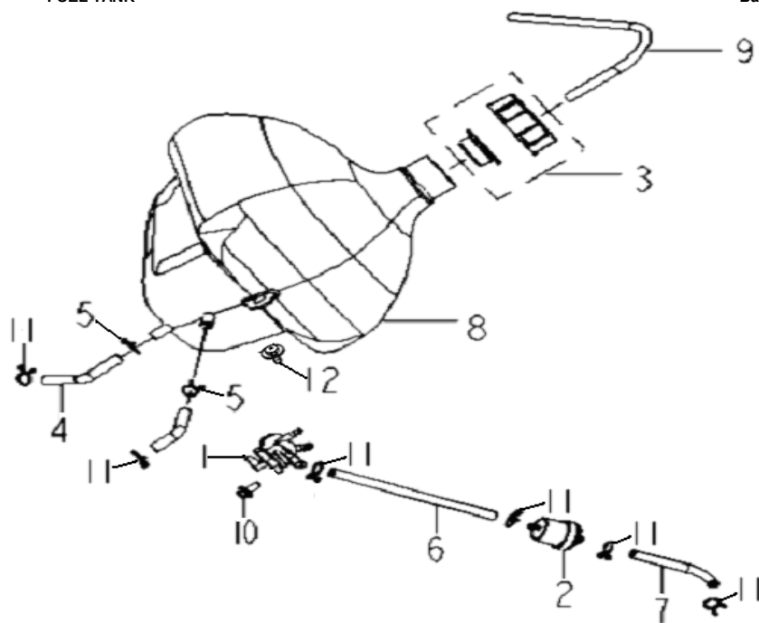
FUEL TANK
