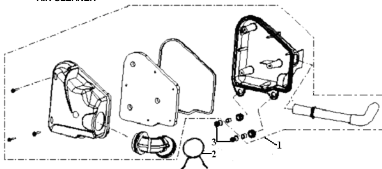
AIR CLEANER
