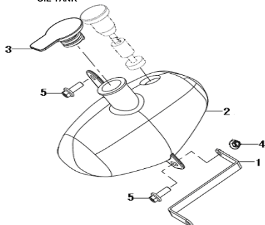
OIL TANK
